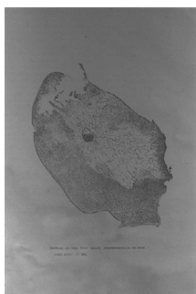
Section of the Kôji grain perpendicular to the long axis. x 364. 麴粒の長軸の垂直切片. 364倍
