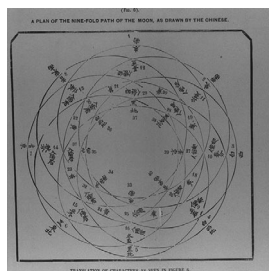
A plan of the nine-fold path of the moon, as drawn by the Chinese.
