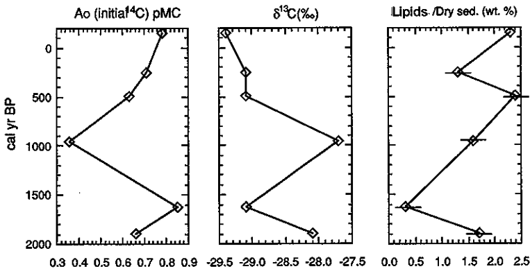
Fig. 2. Initial radiocarbon contents (Ao), \delta^{13}\text{C} and contents of lipids in sediment from Lake Kestel as a function of calibrated ^{14}\text{C} age.
